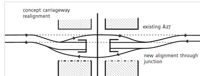
Figure 21. Stockbridge Junction – Concept Junction and Slip Road Approaches (2)
