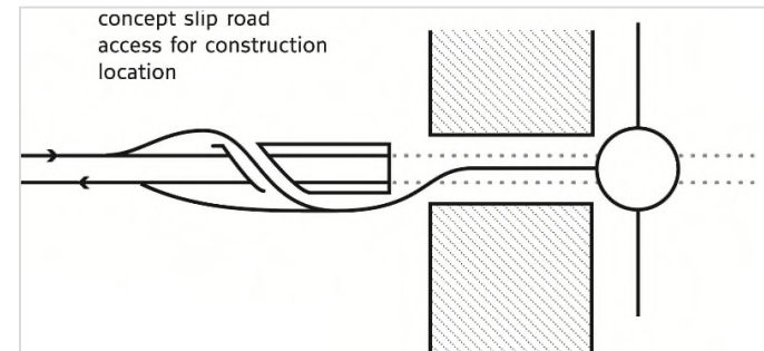
Figure 20. Stockbridge Junction – Concept Junction and Slip Road Approaches (1)
