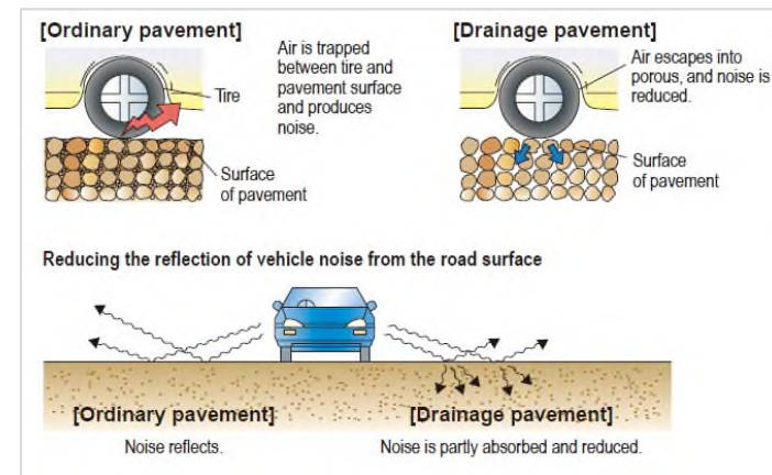
Figure 17. Noise Reducing Asphalt
