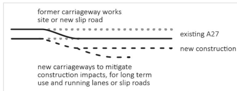
Figure 23. Carriageway Realignments to Provide Space for Slips Roads/Works Sites
